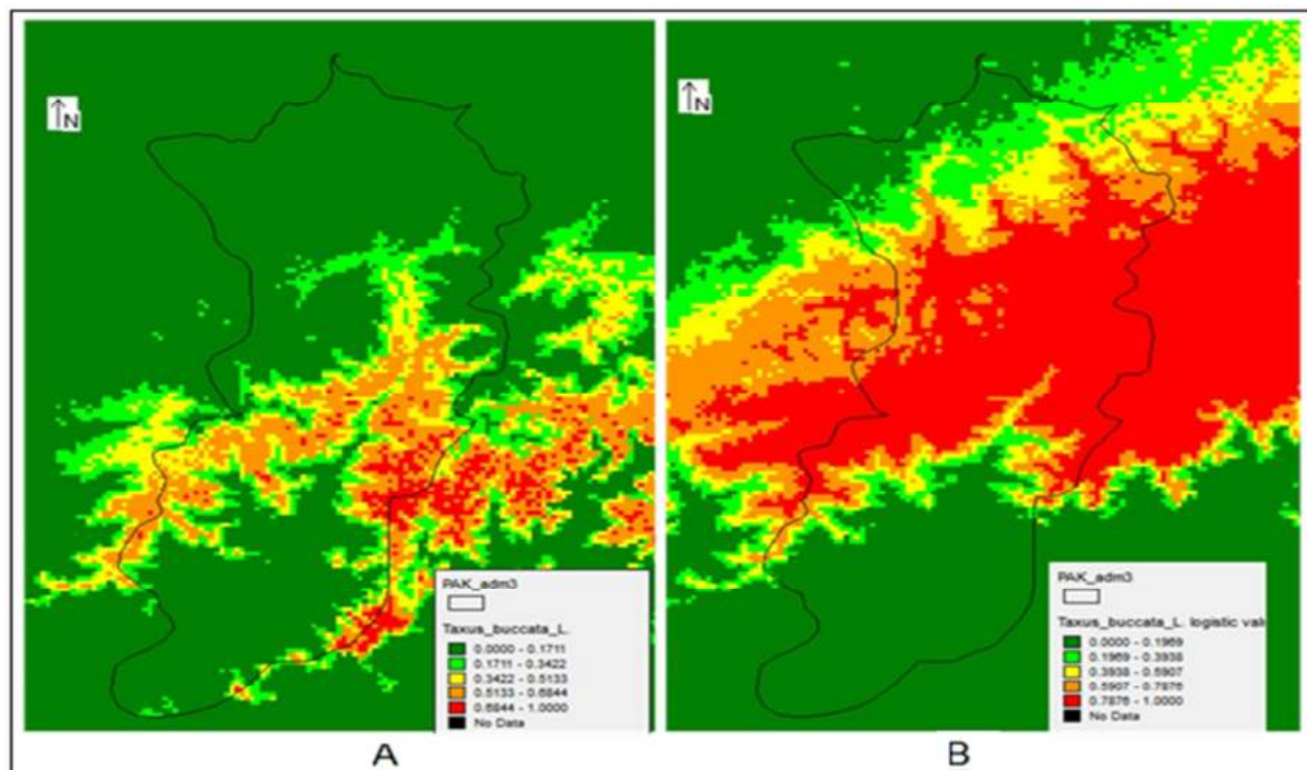
Fig. 10. A. Present distribution of Taxus baccata ; B. Future projection of T. baccata .
