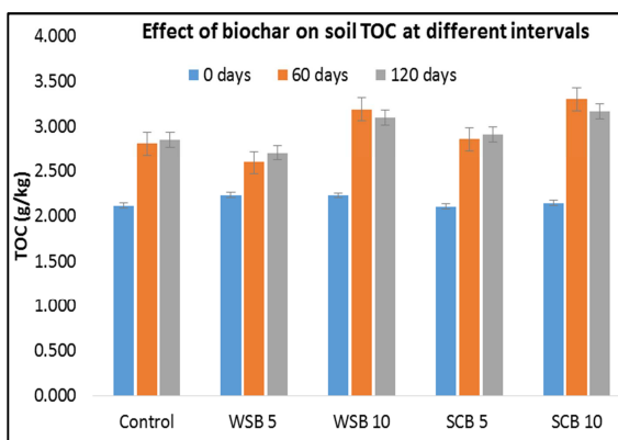
Fig. 3. Data of biochar on soil TOC at different intervals.
