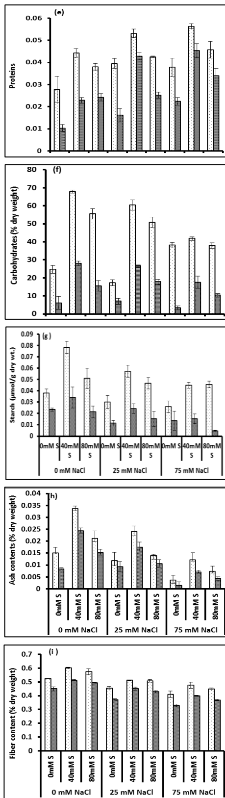
Fig. 2. Effect of different levels of sulfur (S) on leaf \text{PO}_4^{2-} (a) leaf \text{SO}_4^{2-} (b) leaf \text{K}^+/\text{Na}^+ ratio (c) leaf \text{Ca}^{2+}/\text{Na}^+ ratio (d) proteins (e) carbohydrates (f) starch (g) ash contents (h) and fiber contents (i) of different maize ( Zea mays L.) cultivars under saline conditions.
