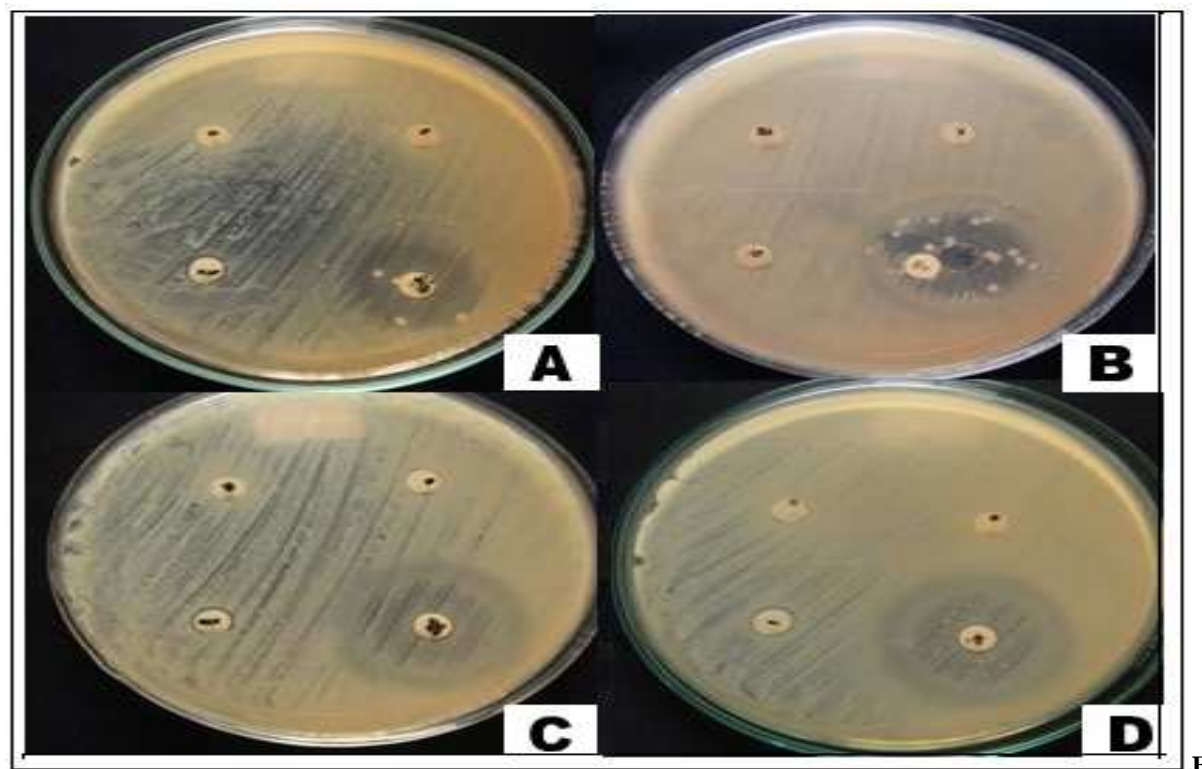
fig. 4. Test for antibacterial activity of different concentrations of decoction preparation of male seahorse using disc diffusion method. Varied concentrations of the decoction preparation: (A) 10% (left), 25% (right); (B) 30% (left) tested against B. subtilis ; (C,D) 10% (left), 25% (right); 30% (left), 70% (right) tested against S. aureus . Tetracycline as positive control (positioned on the lower right most part of the plate) and distilled water as negative control (positioned on the lower right most part of the plate).
