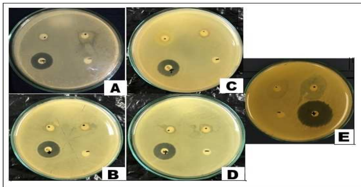
Fig. 1. Test for antibacterial activity of different concentrations of pure crude extract preparation of female pipefishes ( C. intestinalis ) using disc diffusion method. Varied concentrations of the crude extraction: (A) 10% (left), 25% (right) tested against B. subtilis ; (B) 30% (left), 70% (right) tested against B. subtilis ; (C) 10% (left), 25% (right) against P. aeruginosa ; (D) 30% (left), 70% (right) tested against P. aeruginosa ; Tetracycline as positive control (positioned on the lower left most part of the plate) and distilled water as negative control (positioned on the lower right most part of the plate); (E) 30% (left), 70% (right) tested against E. coli after 72 hours of incubation. Tetracycline as positive control (positioned on the lower right most part of the plate) and distilled water as negative control (positioned on the lower left most part of the plate).
