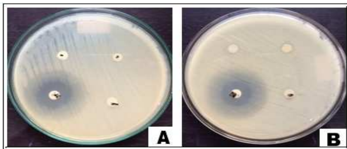
Fig. 2. Test for antibacterial activity of different concentrations of crude extract preparation of male pipefish using disc diffusion method after 72 hrs of incubation. Varied concentrations of the crude extraction: (A) 25% (right) tested against Pseudomonas aeruginosa , and (B) 30% (left), 70% (right) tested against Staphylococcus aureus . Tetracycline as positive control (positioned on the lower right most part of the plate) and distilled water as negative control (positioned on the lower right most part of the plate).
