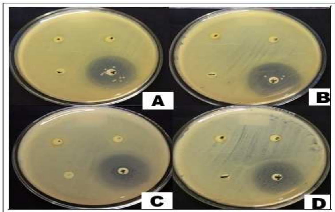
Fig. 3. Test for antibacterial activity of different concentrations of crude extract preparation of male seahorse using disc diffusion method. Varied concentrations of the crude extraction: (A) 10% (left), 25% (right) and (B) 30% (left), 70% (right) on B. subtilis , (C) 10% (left), 25% (right) and (D) 30% (left), 70% (right) on E. coli after 72 hours of incubation. Tetracycline as positive control (positioned on the lower right most part of the plate) and distilled water as negative control (positioned on the lower right most part of the plate).
