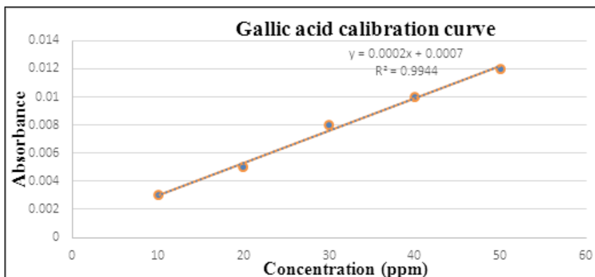
Fig. 1. Gallic acid calibration curve.
