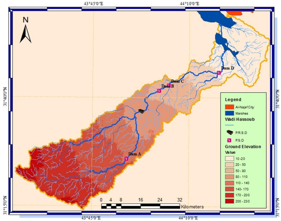
Fig. 4. Wade Hassoub, including the real and proposal submersible dam in the study area.
