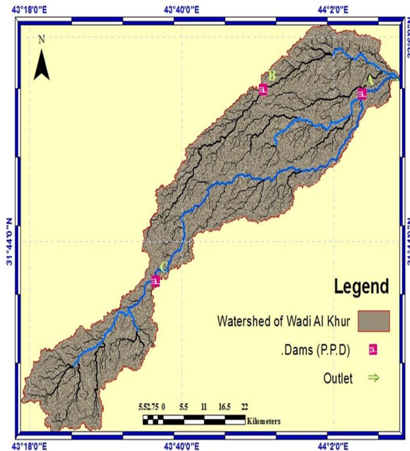
Fig. 3. Wade Al-Khur watershed and positions of proposal submersible dams. P.P.D: position of proposal dams.
