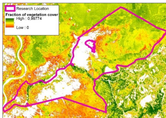
Fig. 6. FVC imagery.
