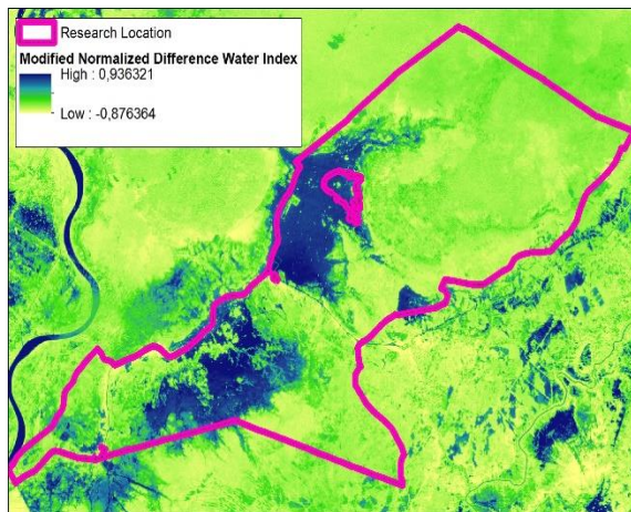
Fig. 10. MNDWI imagery.
