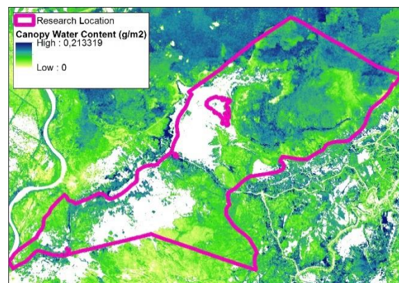
Fig. 9. CWC imagery.
