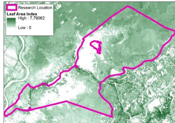
Fig. 5. LAI imagery.
