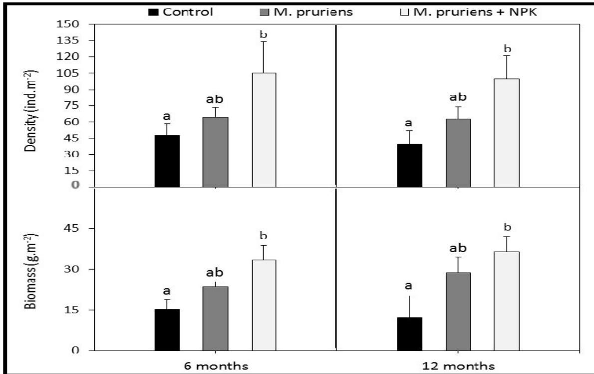
Fig. 1. Overall earthworm community density and biomass after six and 12 months of following. Significant differences between treatments are indicated by different letters ( p < 0.05 ).
