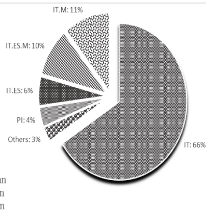
Fig. 2. Plant chorotypes and their relative percentage in flora of winter and rural rangelands in Northern Azarbaijan province.
