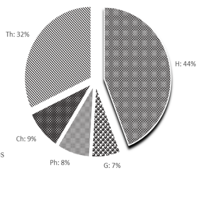
Fig. 3. Plant life forms and their relative contribution (percent) in flora of winter and rural rangelands in Northern Azarbaijan Province.
