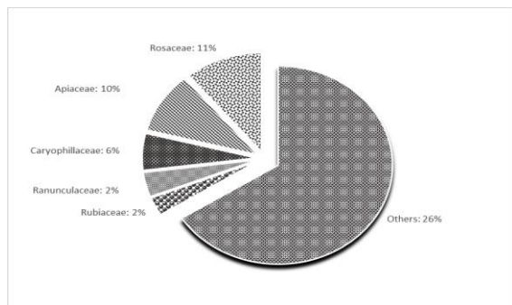
Fig. 4. Proportional contribution of plant families in flora of winter and rural rangelands in Northern Azarbaijan Province; Others: families less than 2% abundance.
