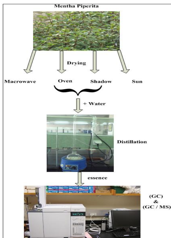
Fig. 2. Process diagram.
